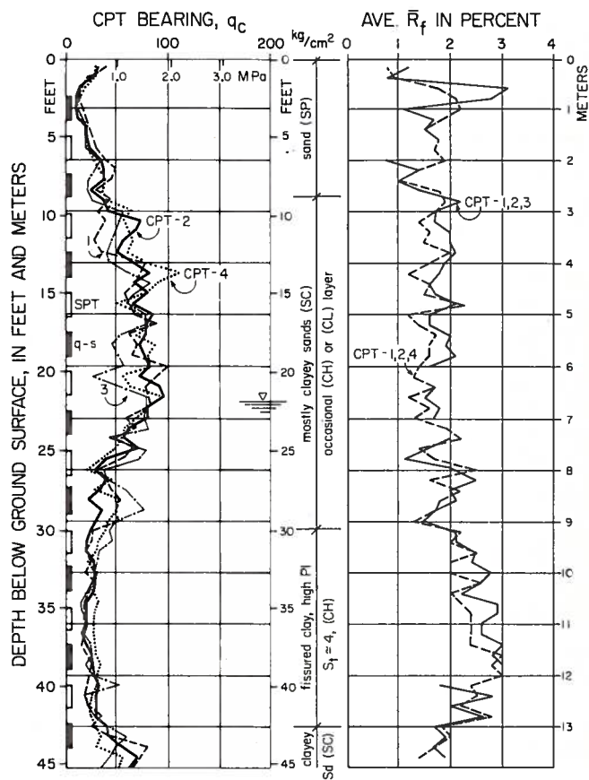
FIG. 3.—Logs of q_c and Average R_f Data from CPT Fig. 2, Also Showing Alternate Depths of Parallel Q-S and N-SPT
