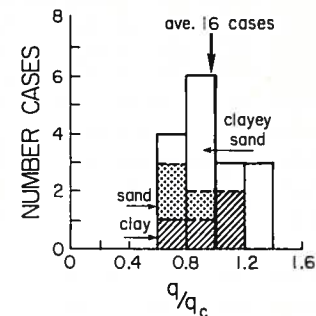
FIG. 5.—Comparison of End Bearing on SPT Sampler and CPT Begemann Cone Tip
